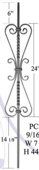
SQUARE PC28/5 1/2" Sq. H 44 3/32" PLAIN PC28/6 9/16" Sq. H 44 3/32" PLAIN PC28/7 5/8" Sq. H 44 3/32" PLAIN
